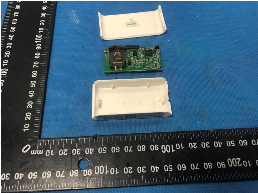
Photo 6: Internal view
